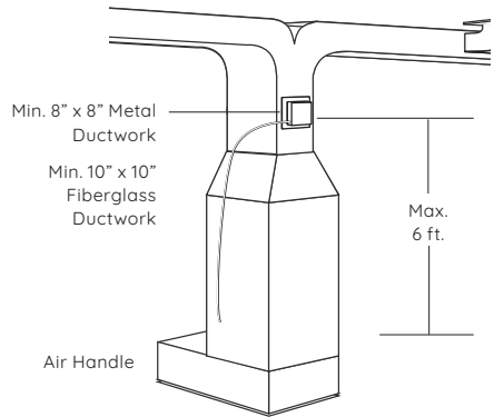
Installation Clearance
